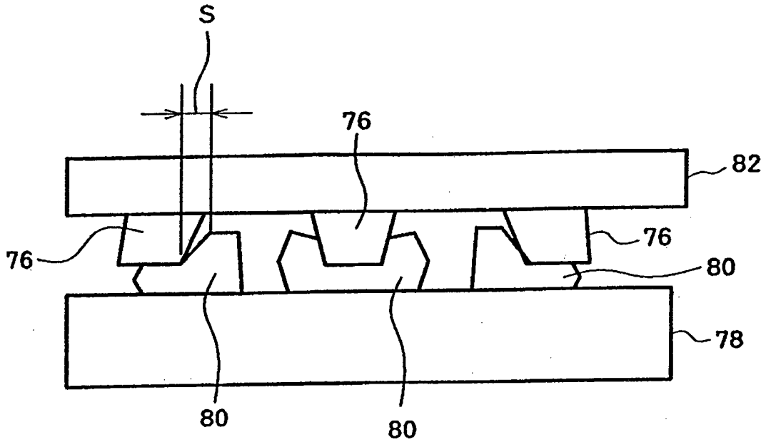
FIG. 10 PRIOR ART
